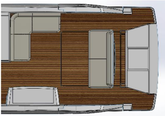
Layout 1A Central aft seat with 2 entrances Gourmet inside
