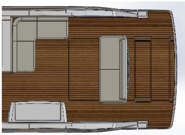
Layout 3A Central aft seat with 2 entrances Gourmet inside
