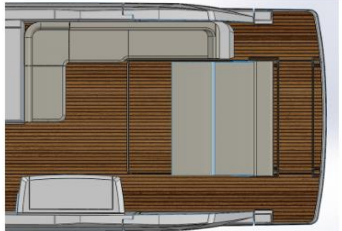
Layout 6A - Open Position Central aft bench shown with actuating back rest folded down to create one large sunpad.
