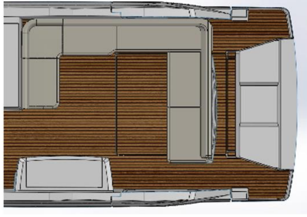
Layout 1F U-shaped seat and 1 entrance Gourmet inside
