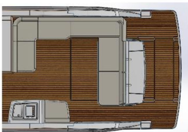
Layout 5F U-shaped seat and 1 entrance Gourmet facing the swim platform Small gourmet inside + seat
