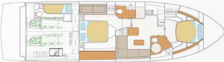
CABINS - OPTION 1
