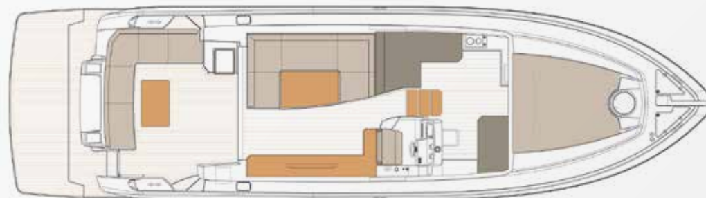
MAIN DECK - OPTION 1
